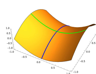
“good” saddle points
